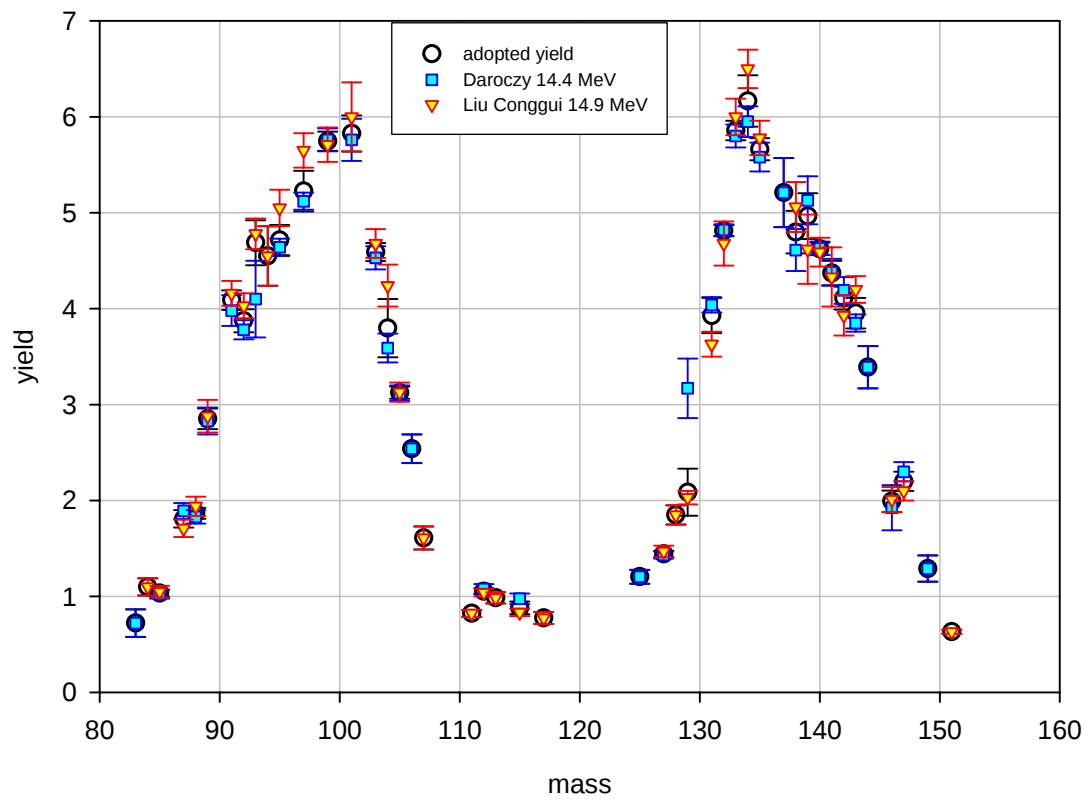
Benchmark A: ^{238}\text{U} around 14.5 MeV, post neutron emission experimental yield
